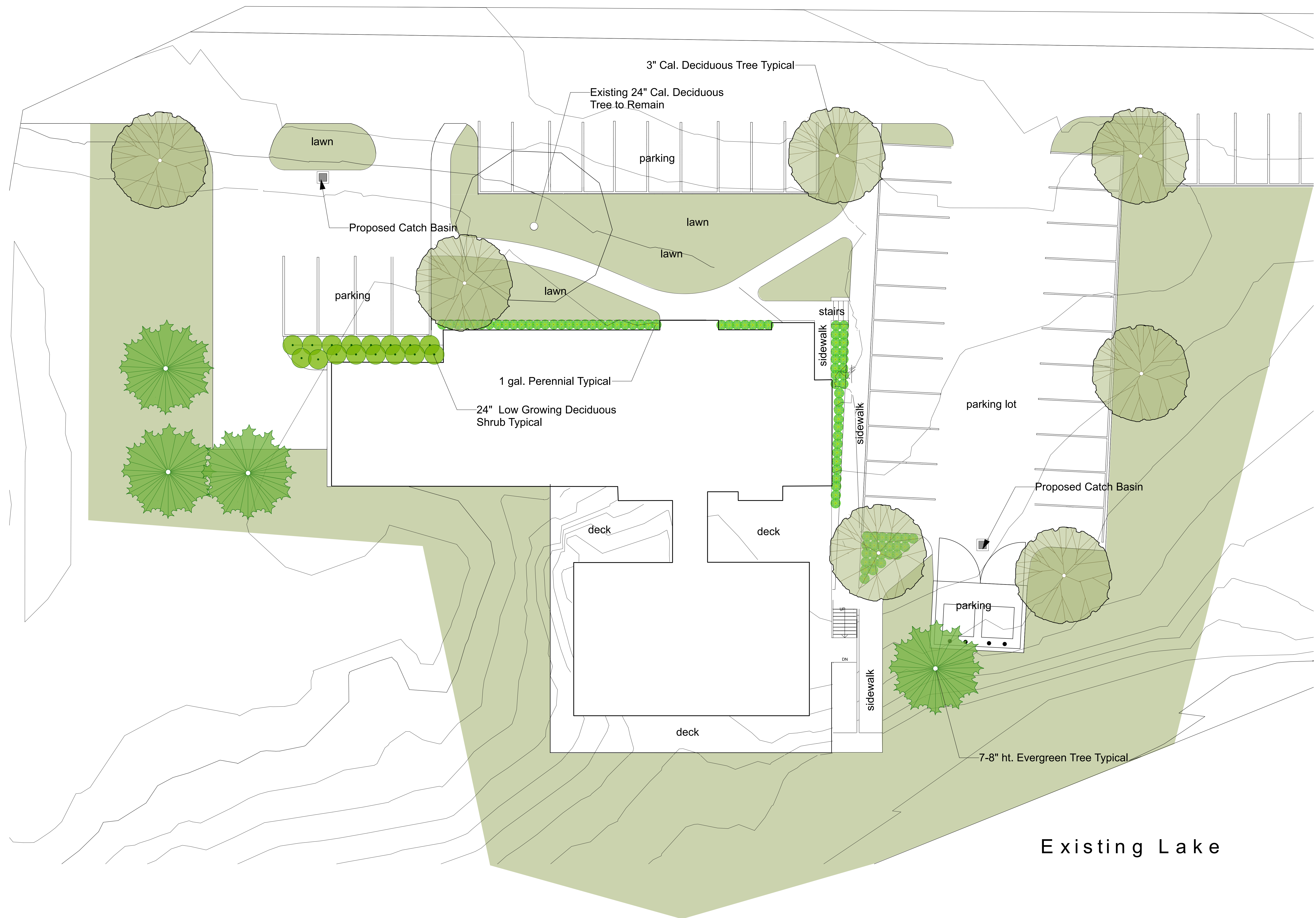
Landscape Plan Scale: 1" = 10'-0"
